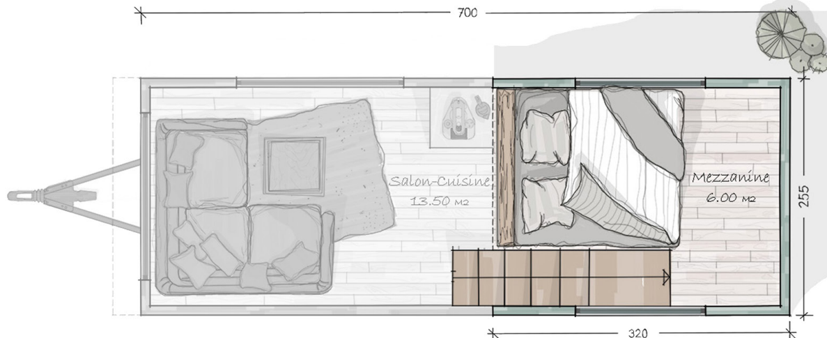
PLAN SUN-HUGE- (26 m 2 )
